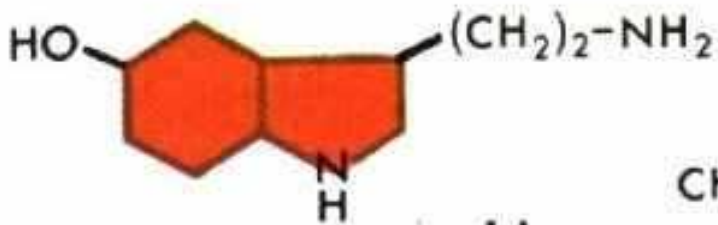
Serotonin
