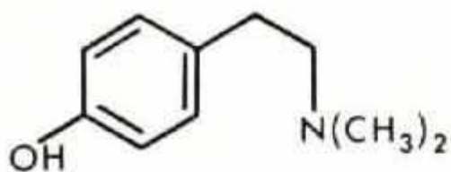
Anhaline
