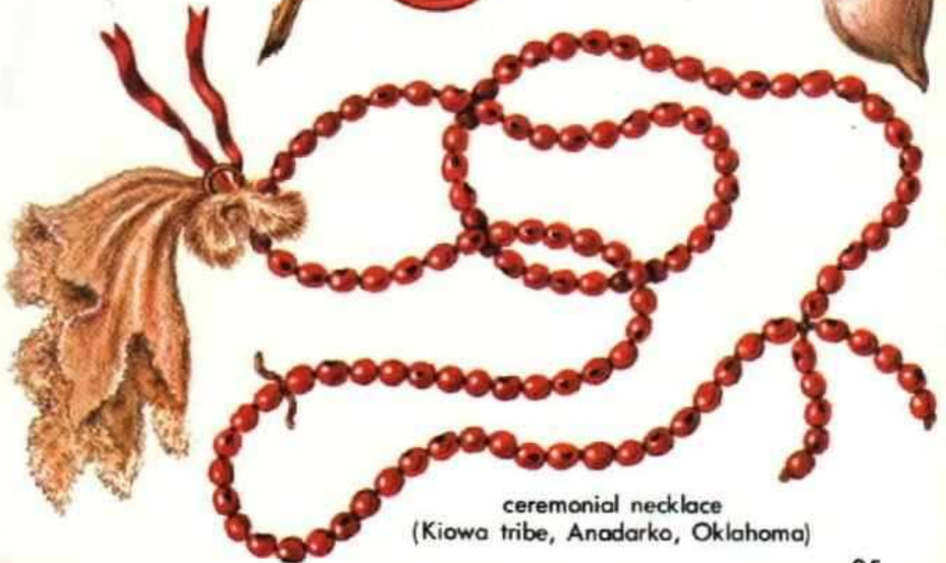
seed
