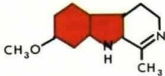
Harmaline
