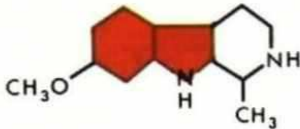
Tetrahydroharmine
