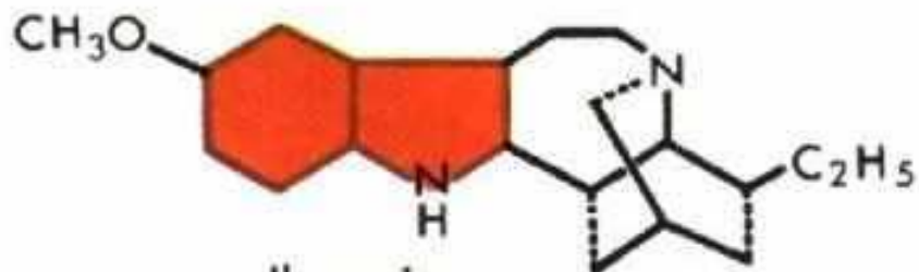
Ibogaine
