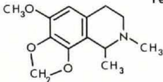
Lophophorine
