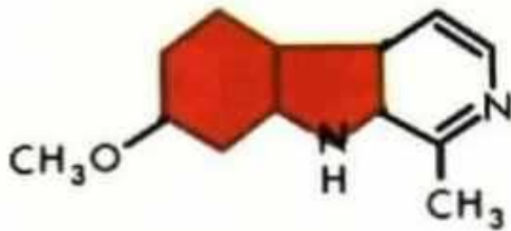
Harmine
