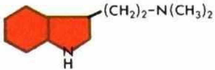
N,N = Dimethyltryptamine
