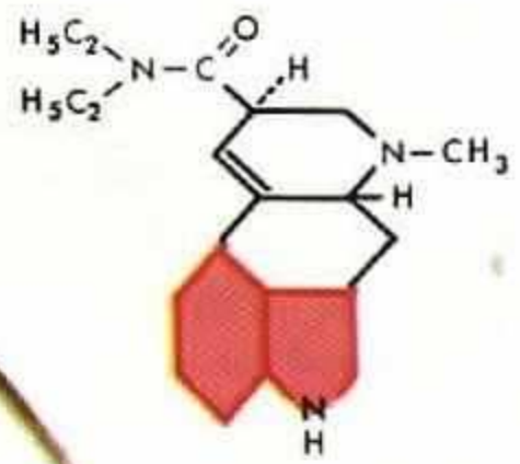
LSD 25
