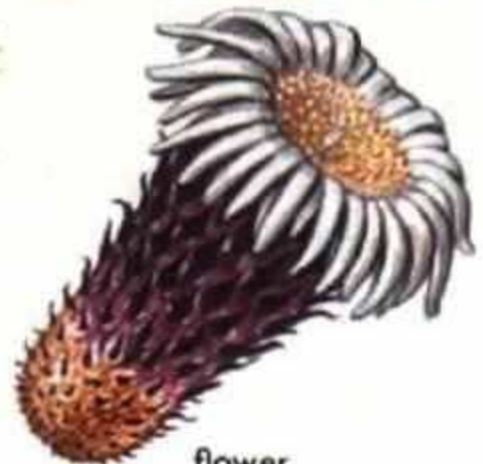
flower
