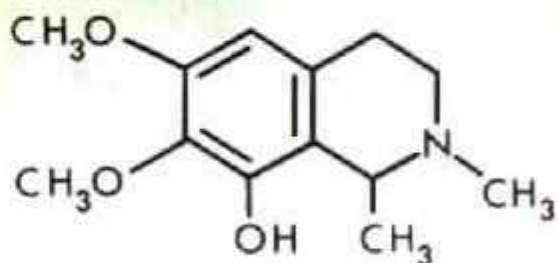
Pellotine
