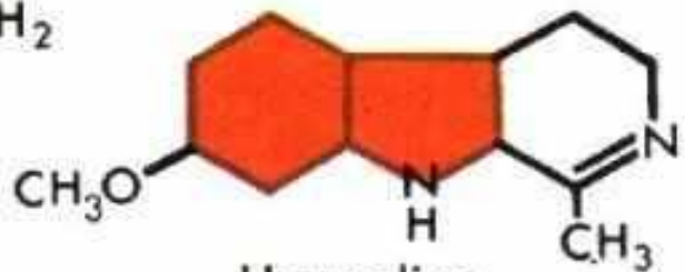
Harmaline
