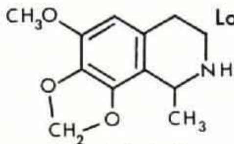
Anhalonine
