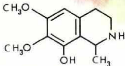
Anhalonidine
