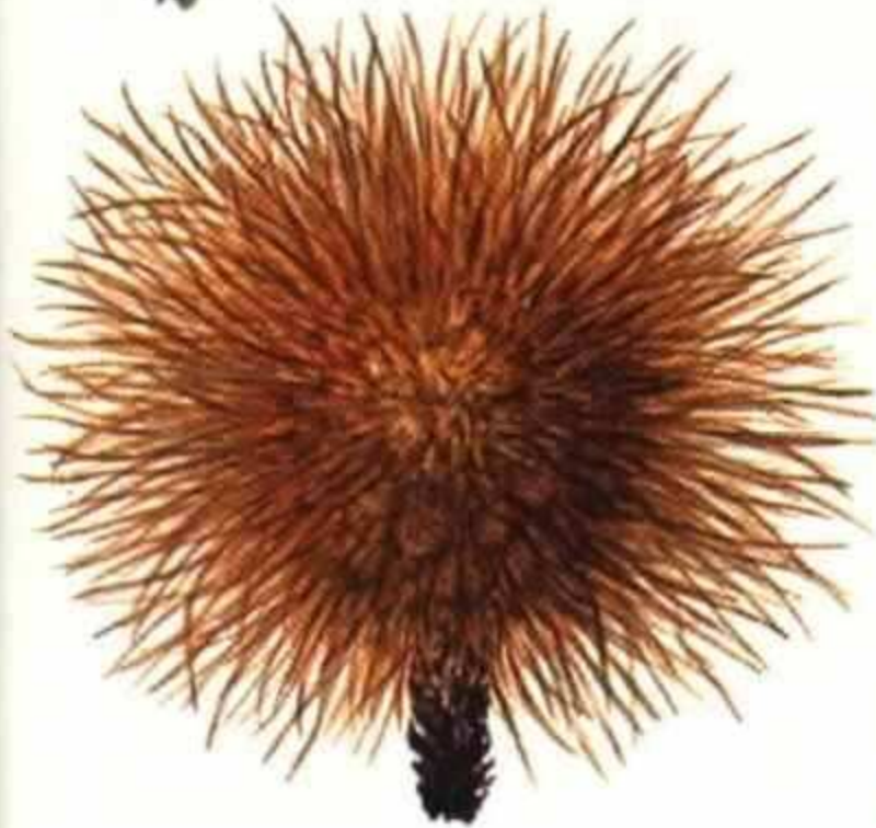
fruit
