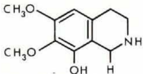
Anhalamine
