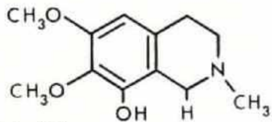
Anhalidine
